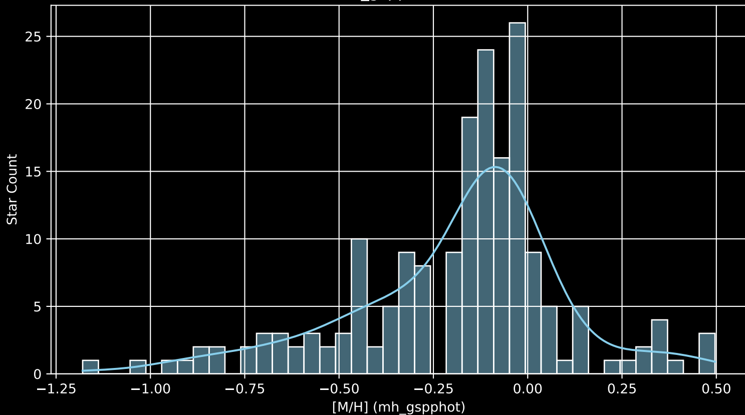
APOGEE DR17 Field: [180-45 [M/H] (mh_gspphot) (n= 186)
