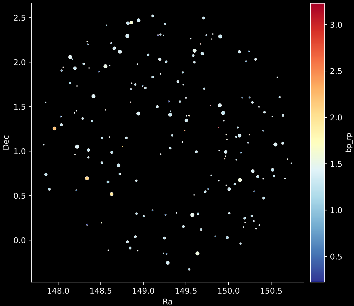
APOGEE DR17 Field: [180-45] Stars: 186
