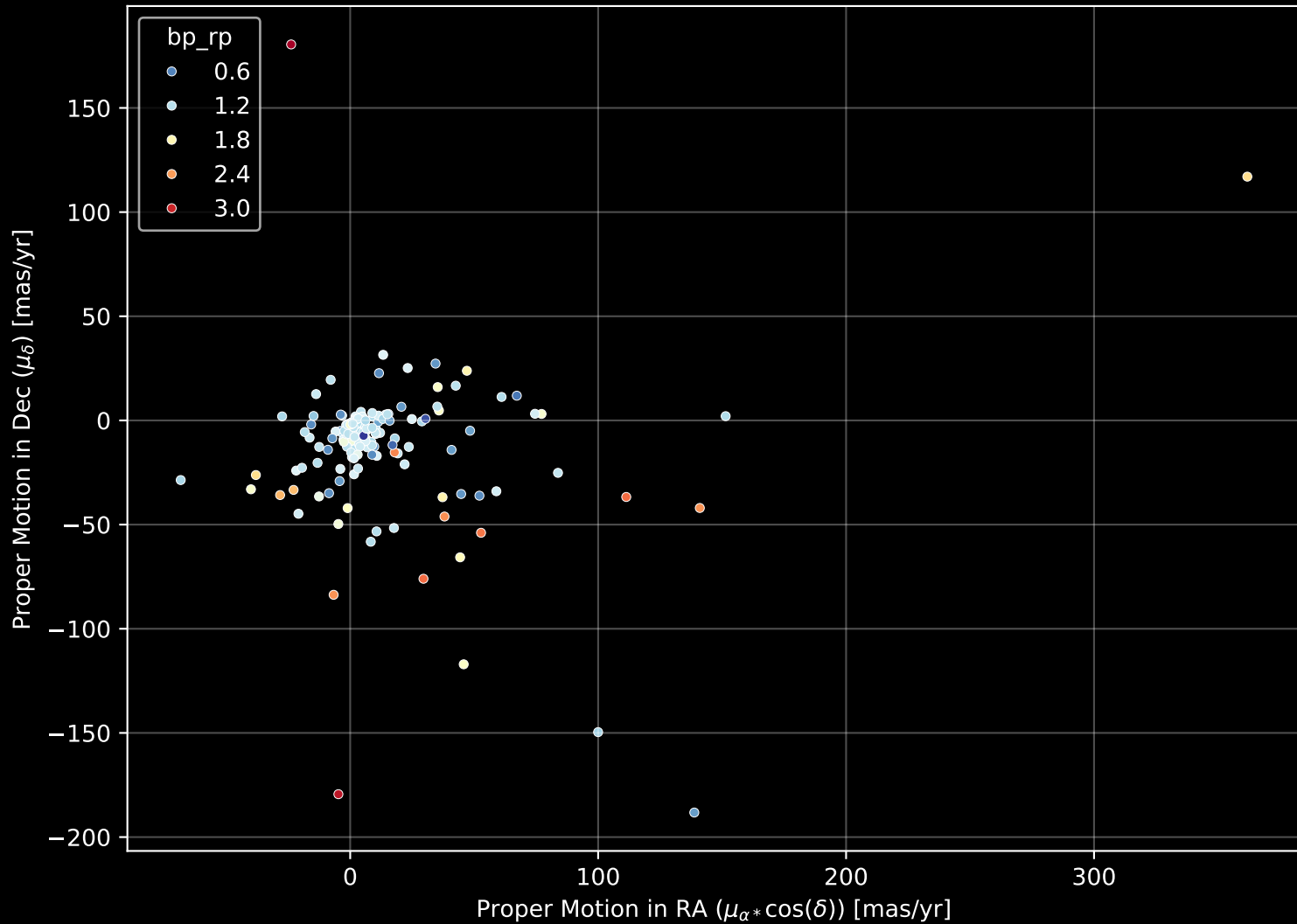
APOGEE DR17 Field: [180-45] Proper Motion Diagram (n= 186)
