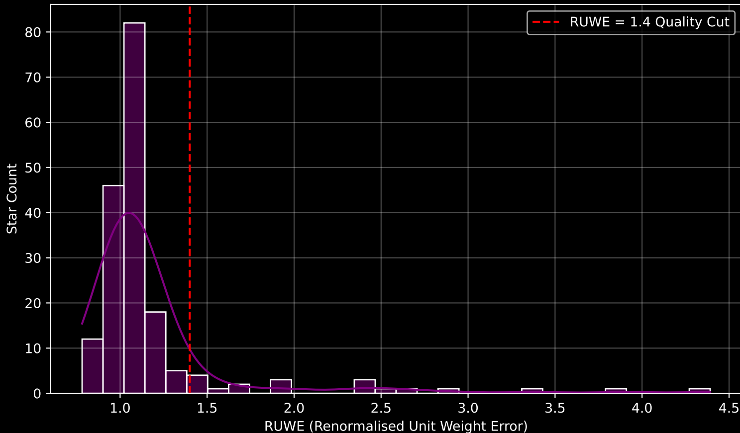
GAPOGEE DR17 Field [180-45] RUWE Distribution (n= 182)
