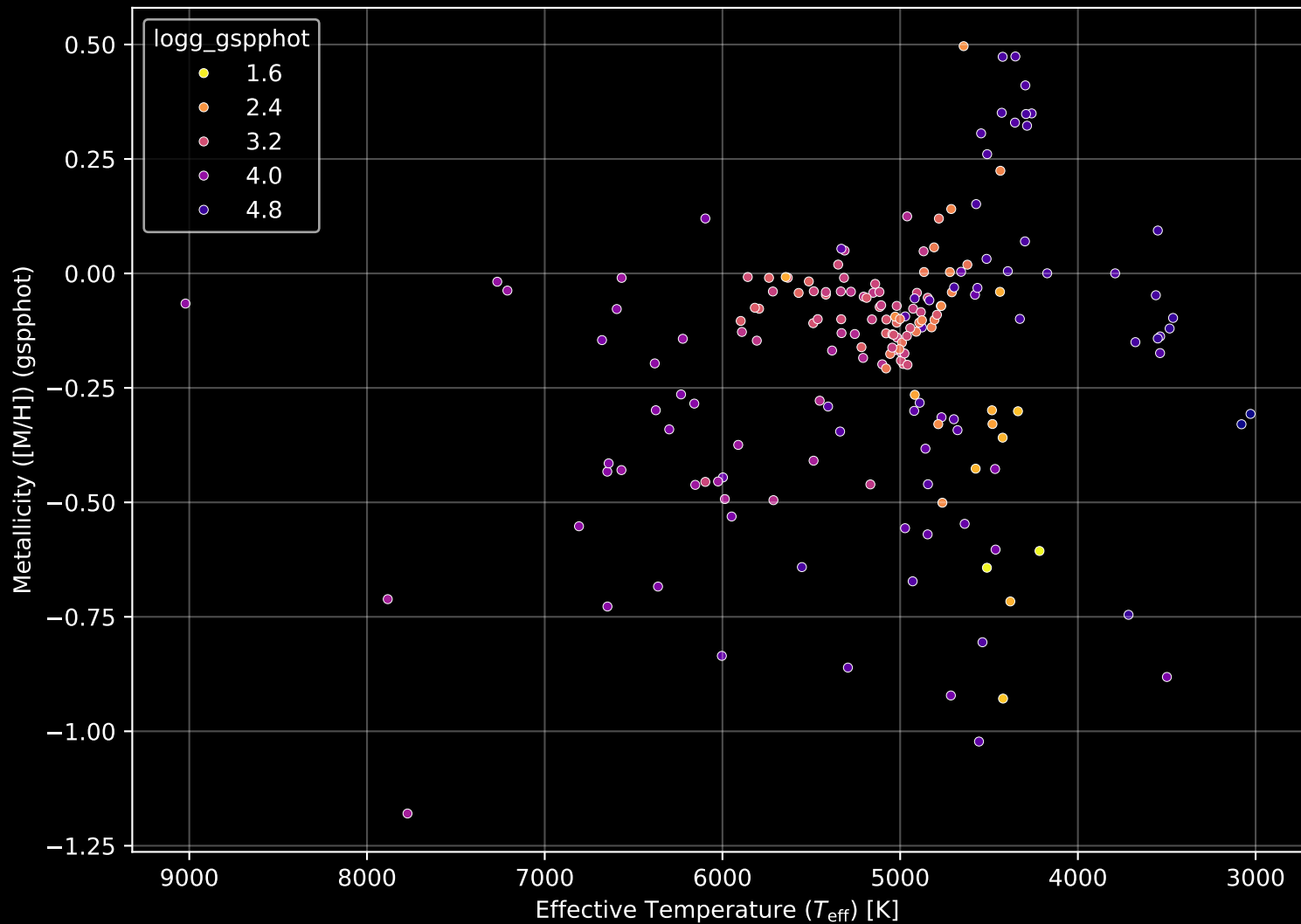
APOGEE DR17 Field: [180-45] Stellar Population Parameters (n= 186)
