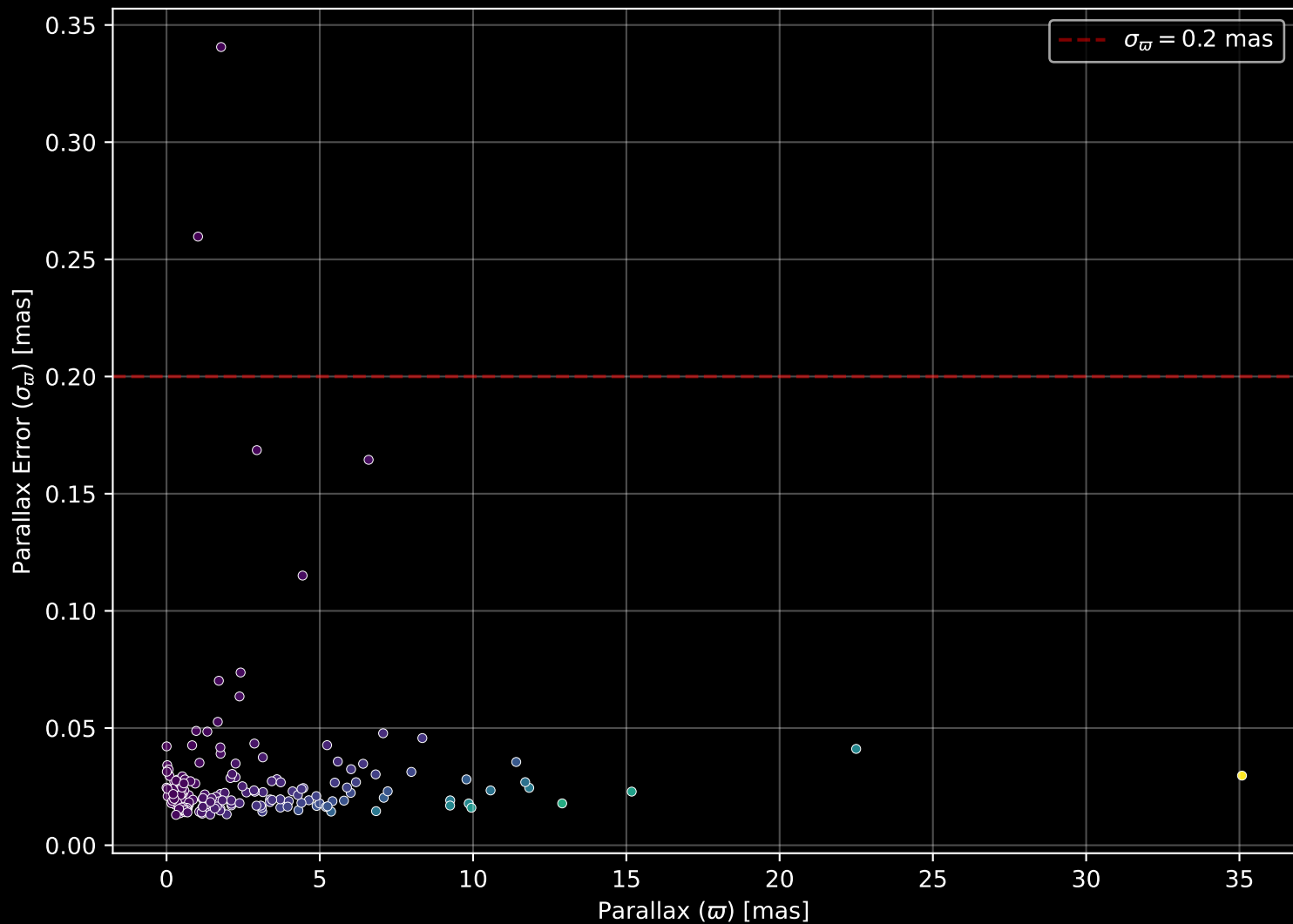
APOGEE DR17 Field: [180-45] Parallax Quality (n= 186)
