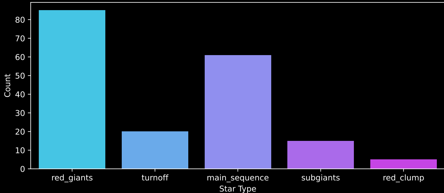
APOGEE DR17 Field: [180-45] Count plot of Star Type
